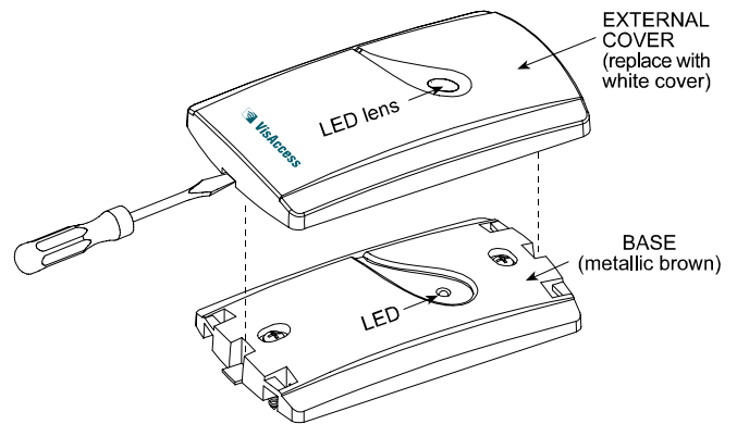
Figure 2 - Cover Removal
